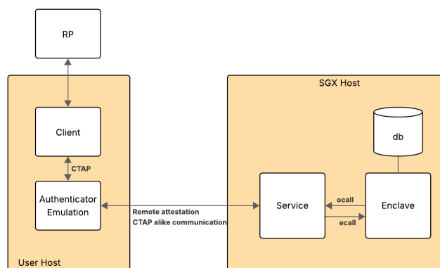
Fig. 1. Architecture of our SGX-based FIDO2 credential manager. The Client application would normally be a browser.
